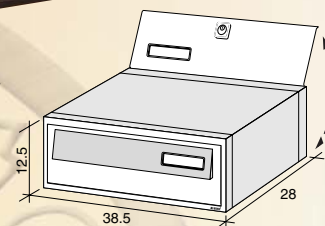
Modular 2 Completa Modular 2 Complete set
