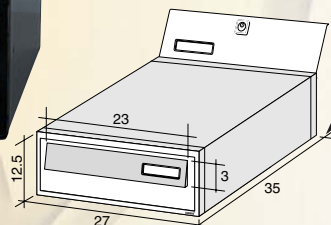
SP270/2R - Retro - Rear door
